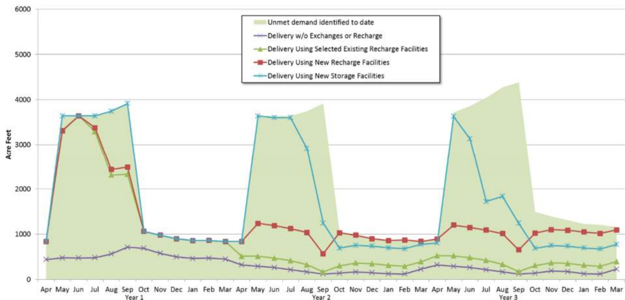
Figure 5-2. Output from Initial Operational Modeling of the NECWC
